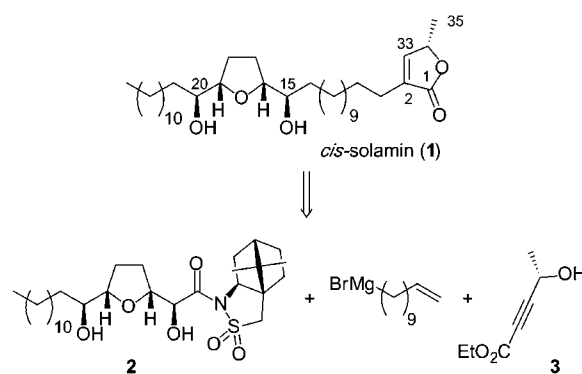
Figure 1. Approach to the synthesis of mono-THF acetogenin cis -solamin ( 1 ).
