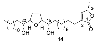
Figure 3. Structure of compound 14 .
