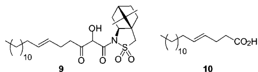
Figure 2. Byproducts from the \text{KMnO}_4 oxidation of diene 7 .
